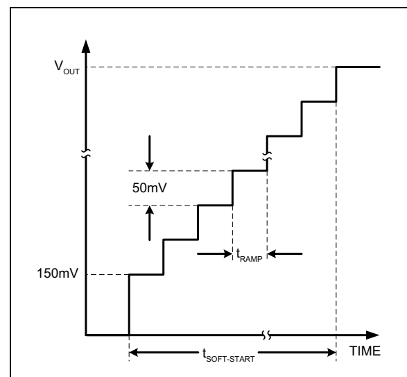
FIGURE 4-1: Buck Soft-Start.
