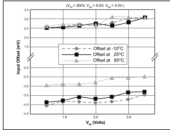
FIGURE 2-10: Input Offset vs. V_{IN} and Temperature.
