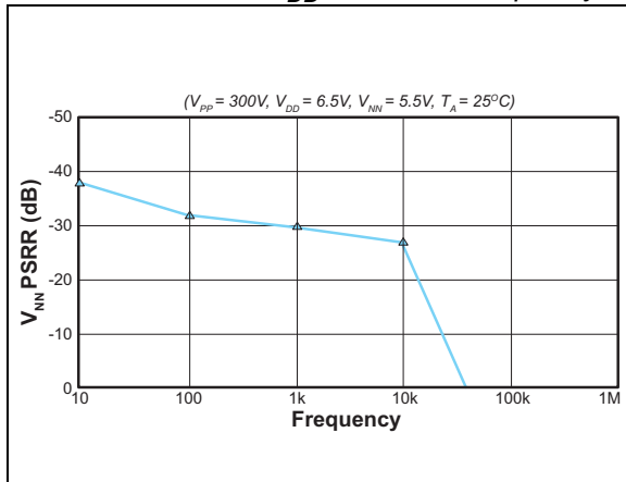
FIGURE 2-9: V_{NN} PSRR vs. Frequency.
