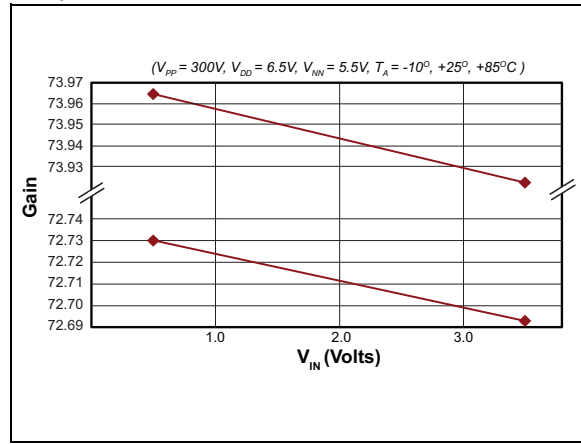
FIGURE 2-11: Gain vs. V_{IN} .
