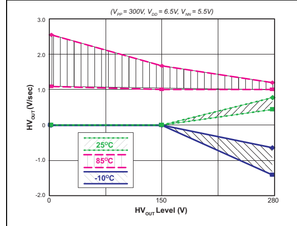
FIGURE 2-6: H_{VOUT} Droop.
