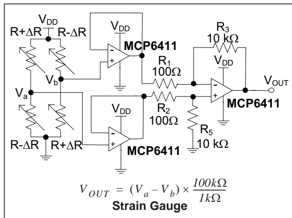
FIGURE 4-8: Pressure Sensor Amplifier.
