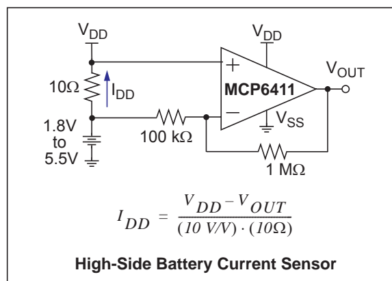
FIGURE 4-9: Battery Current Sensing.
