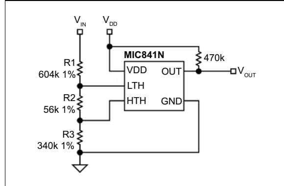
FIGURE 4-1: MIC841 Example Circuit
