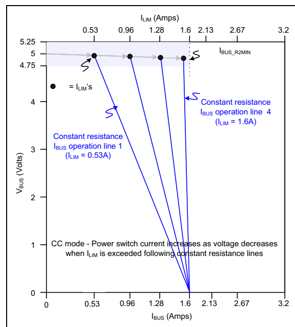
FIGURE 6-3: Current Limiting in CC Mode.
