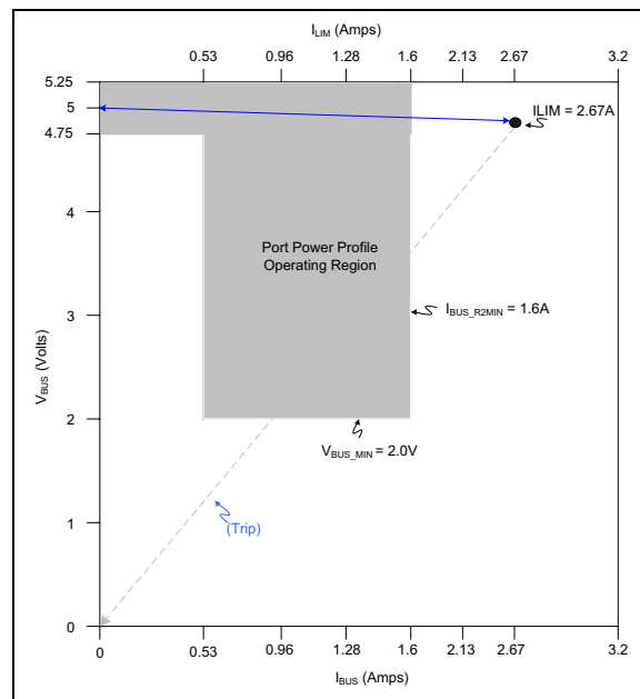
FIGURE 6-5: I_{LIM} > I_{BUS\_R2MIN} Example.
