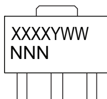
3-lead SOT-89
