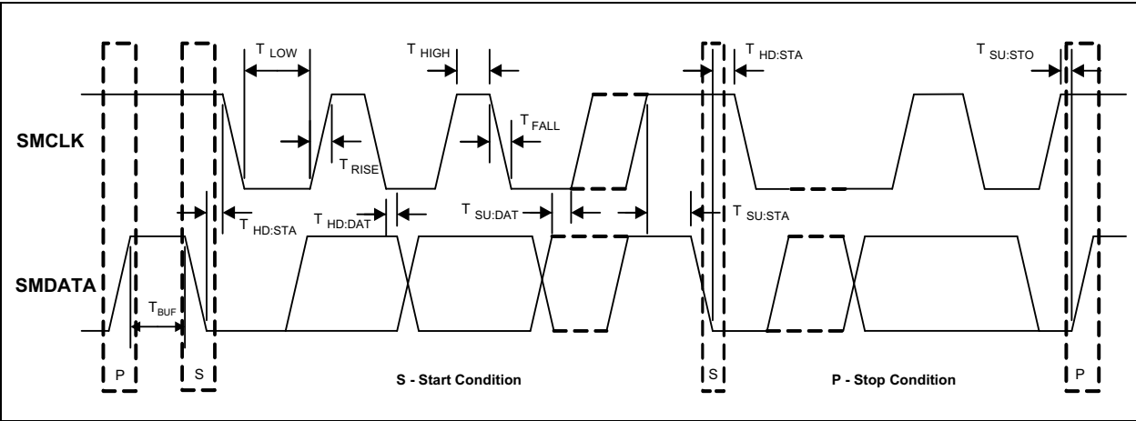
FIGURE 1-1: SMBus Timing.
