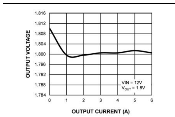
FIGURE 2-20: Output Voltage vs. Output Current.
