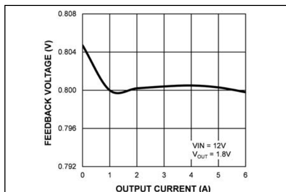
FIGURE 2-19: Feedback Voltage vs. Output Current.
