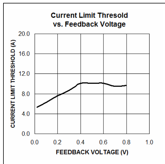
FIGURE 4-4: MIC24052 Current-Limit Foldback Characteristic.
