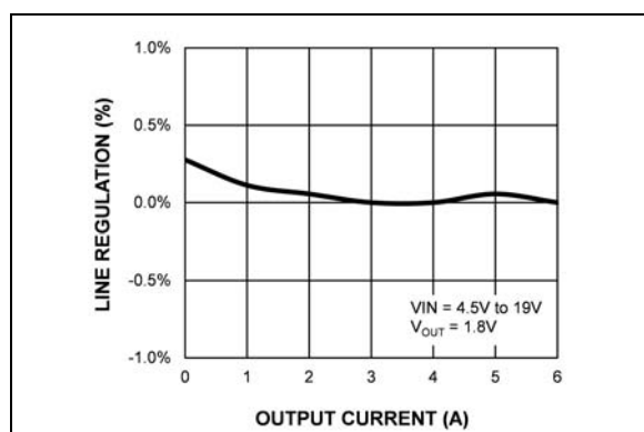
FIGURE 2-21: Line Regulation vs. Output Current.
