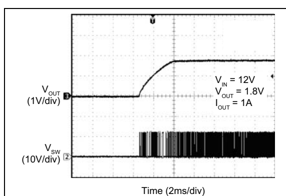
FIGURE 2-47: Output Recovery from Thermal Shutdown.
