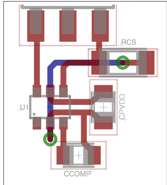
FIGURE 3-2: Connection to the GND Pin.
