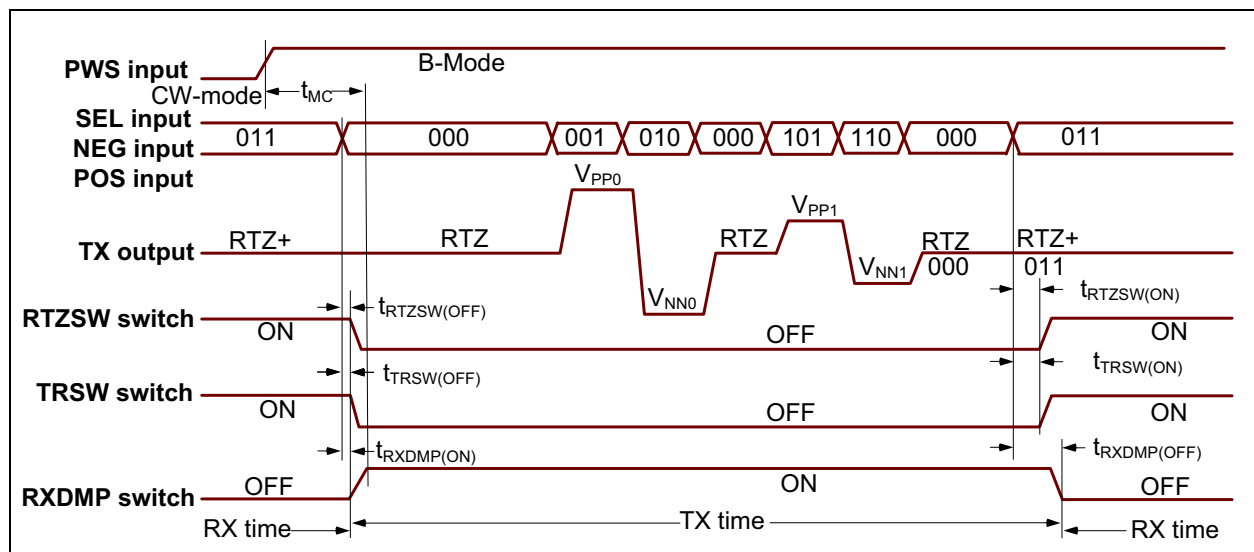
FIGURE 1-2: TX Output Timing Diagram.
