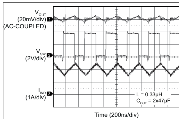
FIGURE 2-37: Switching Waveform Continuous Mode (2A).
