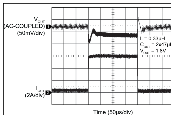
FIGURE 2-30: Load Transient 200 mA to 6A.
