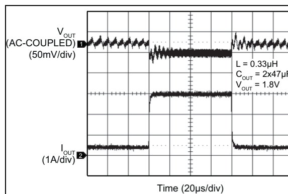
FIGURE 2-29: Load Transient 200 mA to 3A.
