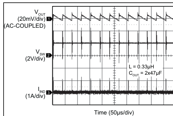
FIGURE 2-34: Switching Waveform Discontinuous Mode (10 mA).
