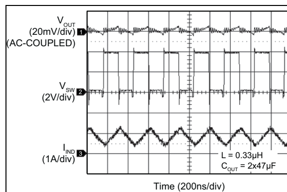
FIGURE 2-36: Switching Waveform Continuous Mode (800 mA).
