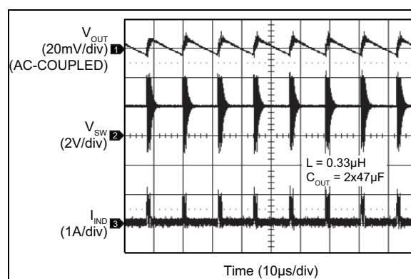
FIGURE 2-35: Switching Waveform Discontinuous Mode (50 mA).
