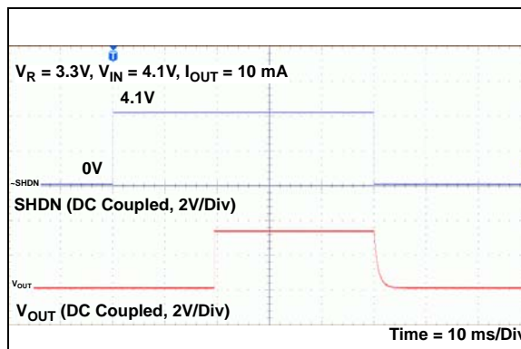
FIGURE 2-34: Start-up from \overline{\text{SHDN}} ( V_R = 3.3\text{V} ).
