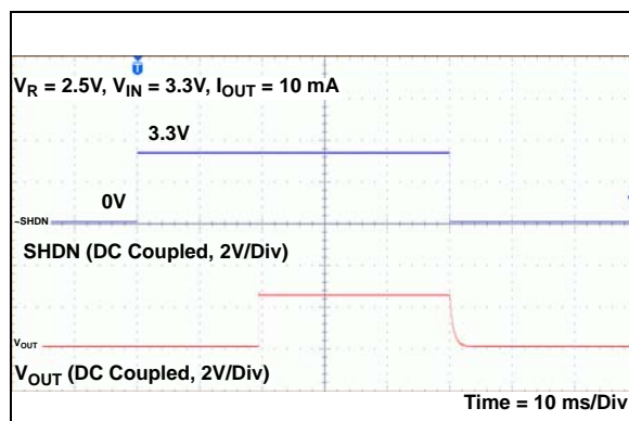
FIGURE 2-33: Start-up from \overline{\text{SHDN}} ( V_R = 2.5\text{V} ).
