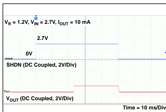
FIGURE 2-32: Start-up from \overline{\text{SHDN}} ( V_R = 1.2\text{V} ).
