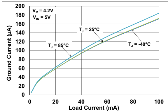
FIGURE 2-55: Ground Current vs. Load Current ( V_R = 4.2V ).
