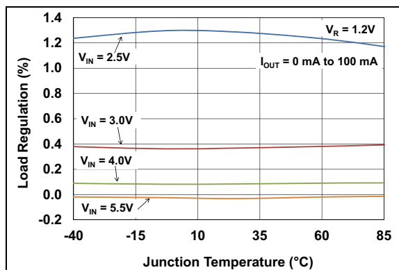
FIGURE 2-36: Load Regulation vs. Junction Temperature ( V_R = 1.2\text{V} ).
