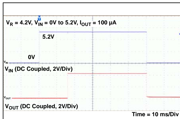
FIGURE 2-31: Start-up from V_{IN} ( V_R = 4.2\text{V} ).
