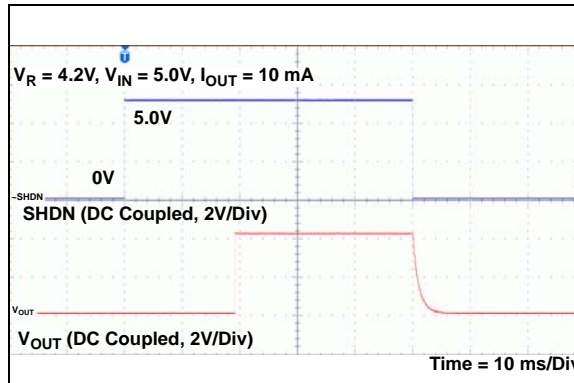
FIGURE 2-35: Start-up from \overline{\text{SHDN}} ( V_R = 4.2\text{V} ).
