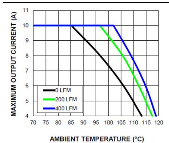
FIGURE 5-7: MIC45208 Power Derating vs. Airflow (12 V_{IN} to 1.5 V_{OUT} ).
