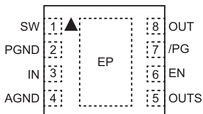
MIC2875 (FIXED OUTPUT) 8-Pin 2x2 TDFN* (MT) (Top View)
