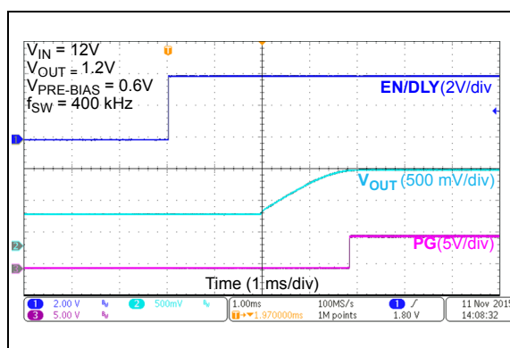
FIGURE 2-22: Enable Start-Up with Pre-Biased Output.
