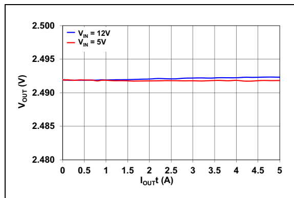
FIGURE 2-16: Output Voltage vs. Output Current ( V_{OUT} = 2.5V ).
