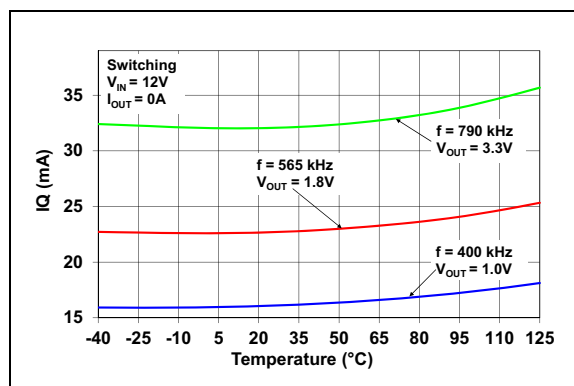
FIGURE 2-6: Operating Current ( I_Q ) vs. Temperature.
