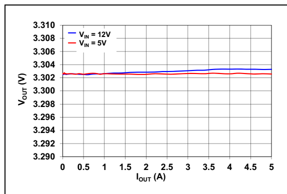
FIGURE 2-17: Output Voltage vs. Output Current ( V_{OUT} = 3.3V ).
