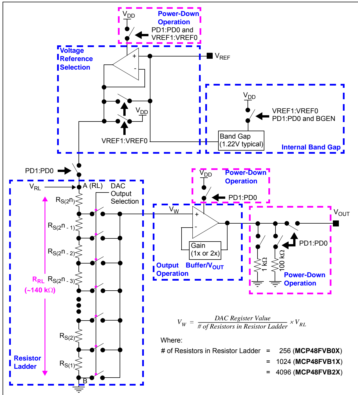
FIGURE 5-1: MCP48FVBXX DAC Module Block Diagram.
