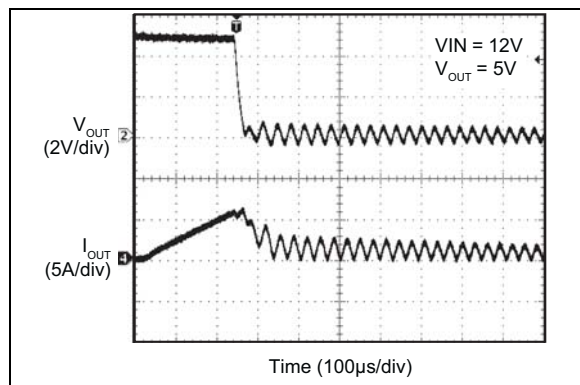
FIGURE 2-49: Short Circuit.
