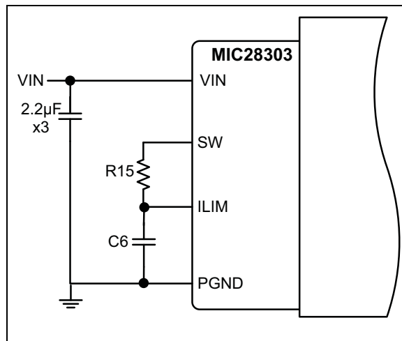
FIGURE 4-4: Current-Limiting Circuit
