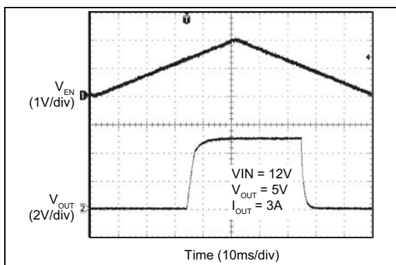
FIGURE 2-44: Enable Thresholds.
