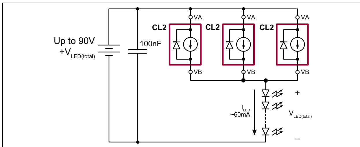
FIGURE 3-5: CL2 for Higher Current
