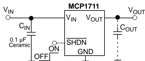
MCP1711 1x1 UQFN and SOT-23
