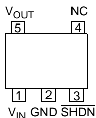
MCP1711 SOT-23 Top View
