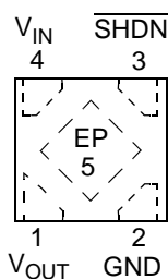
MCP1711 1x1 UQFN* Top View
