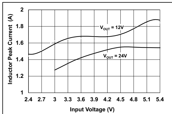
FIGURE 2-7: Inductor Peak Current Limit vs. Input Voltage.
