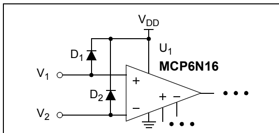
FIGURE 4-8: Protecting the Analog Inputs Against High Voltages.
