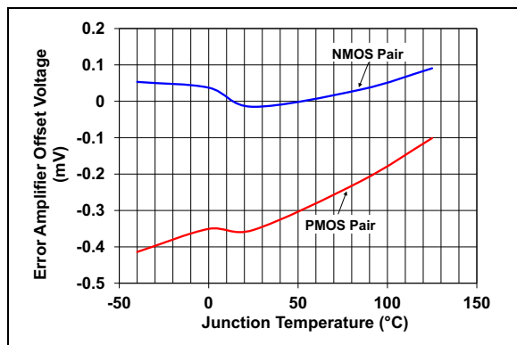
FIGURE 2-7: Error Amplifier Offset Voltage vs. Temperature.
