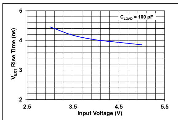
FIGURE 2-9: V_{EXT} Rise Time vs. Input Voltage.
