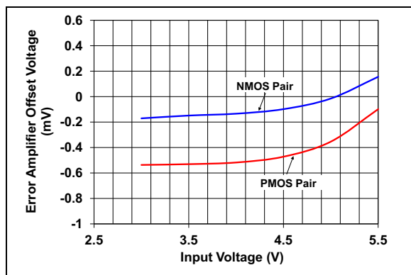
FIGURE 2-8: Error Amplifier Offset Voltage vs. Input Voltage.
