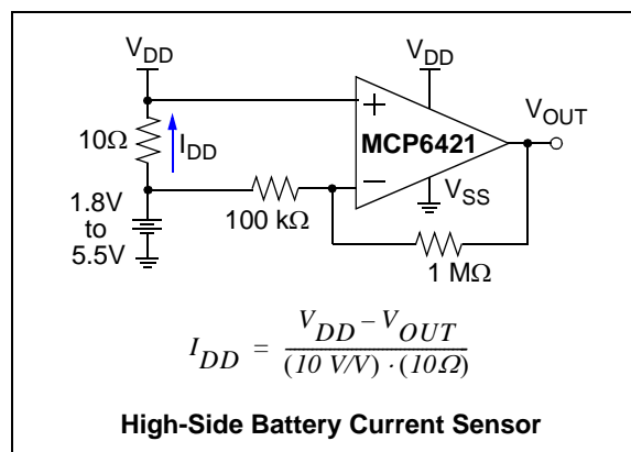
FIGURE 4-10: Battery Current Sensing.
