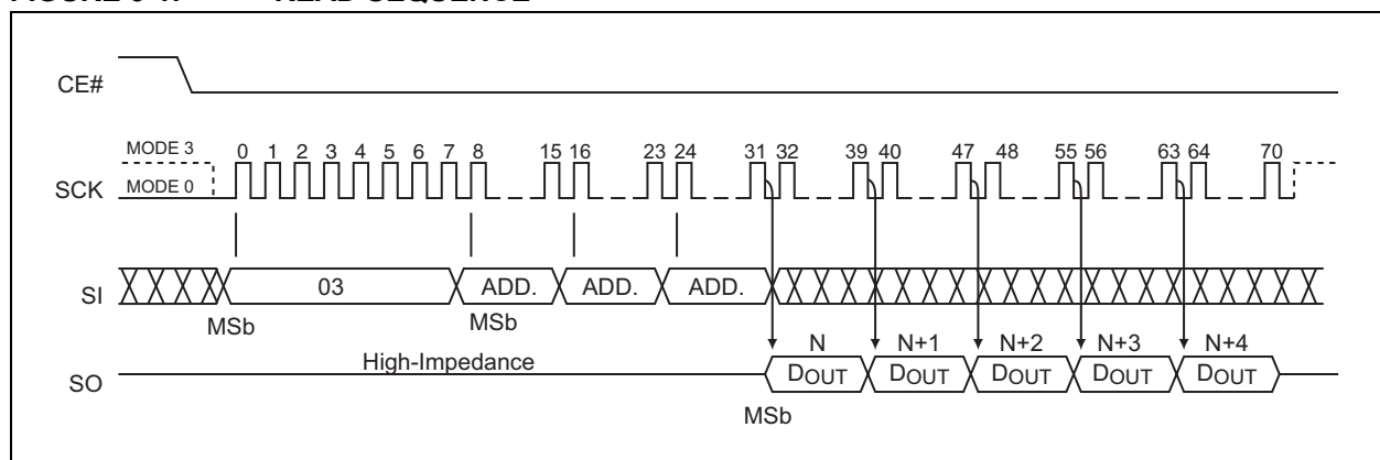
FIGURE 5-1: READ SEQUENCE
