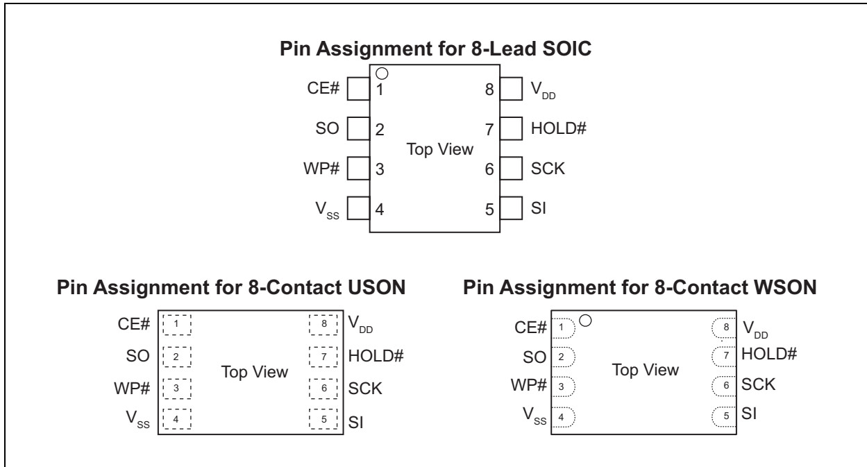
FIGURE 2-1: PIN DESCRIPTIONS
