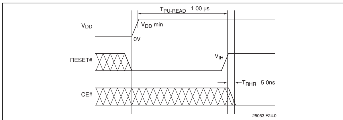
Figure 5: Power-Up Diagram
