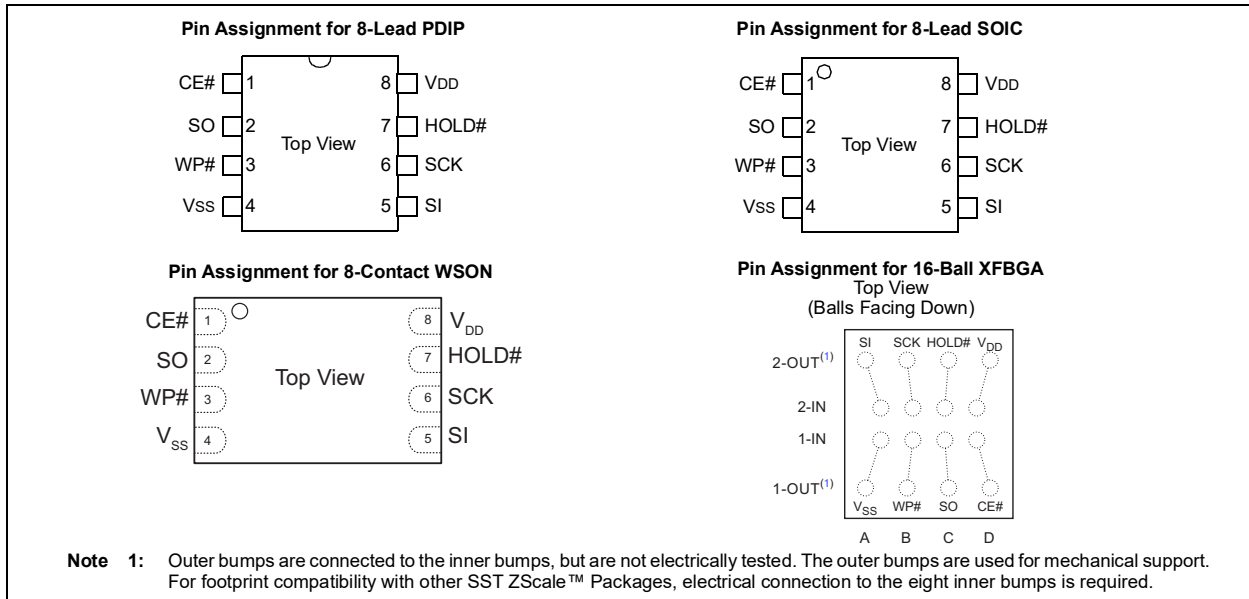
FIGURE 2-1: PIN ASSIGNMENTS
