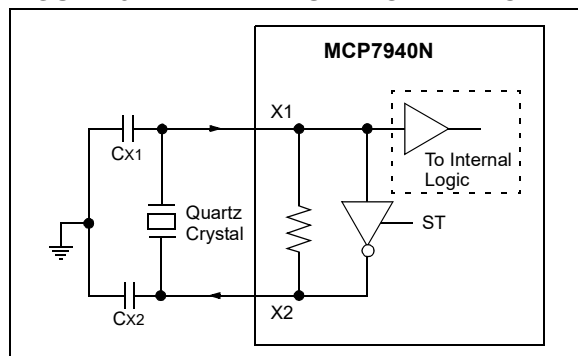
FIGURE 5-2: CRYSTAL OPERATION
