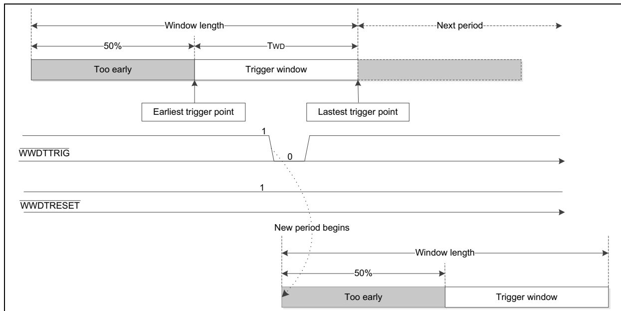
FIGURE 1-3: CORRECT TRIGGER
