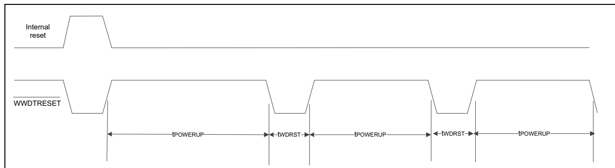
FIGURE 1-2: WWDTRST DURING INITIAL POWER-UP
