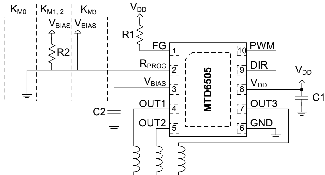
Recommended External Components for Typical Application
