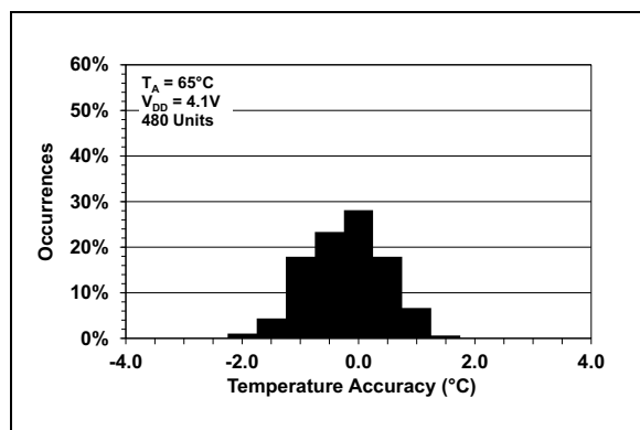
FIGURE 2-9: Temperature Accuracy Distribution at +65^{\circ}C .
