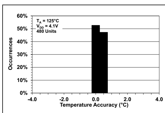
FIGURE 2-12: Temperature Accuracy Distribution at +125^{\circ}C .
