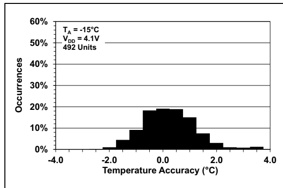
FIGURE 2-7: Temperature Accuracy Distribution at -15^{\circ}C .
