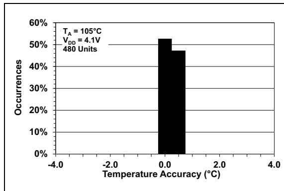
FIGURE 2-10: Temperature Accuracy Distribution at +105^{\circ}C .
