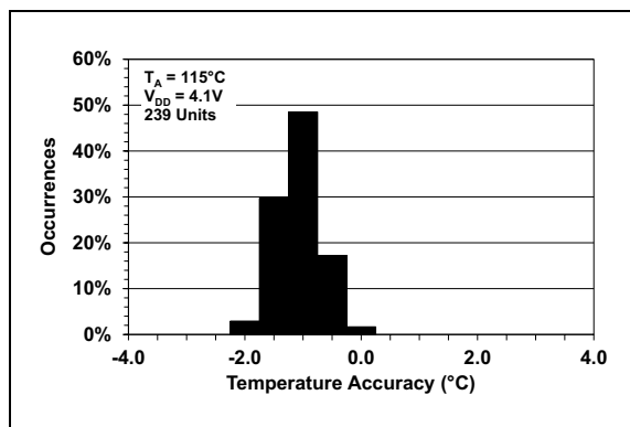
FIGURE 2-11: Temperature Accuracy Distribution at +115^{\circ}C .
