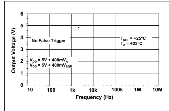
FIGURE 4-6: Power Supply Rejection ( T_{\text{SET}} = +25^{\circ}\text{C} ).
