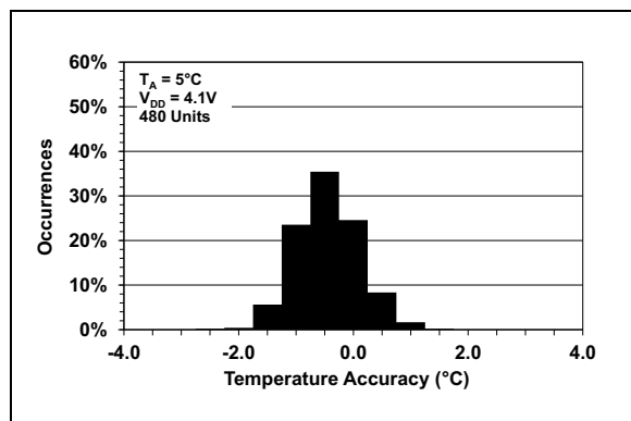
FIGURE 2-8: Temperature Accuracy Distribution at +5^{\circ}C .
