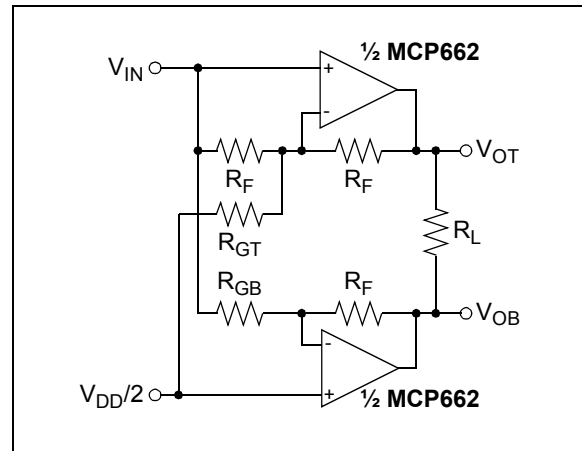
FIGURE 4-12: H-Bridge Driver.
