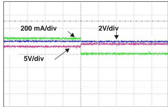
FIGURE 2-16: Input Overvoltage Protection ( V_{IN} = 5V/Div , V_{BAT} = 2V/Div , I_{LOAD} = 200 mA/Div , Time: 200 ms/Div ).
