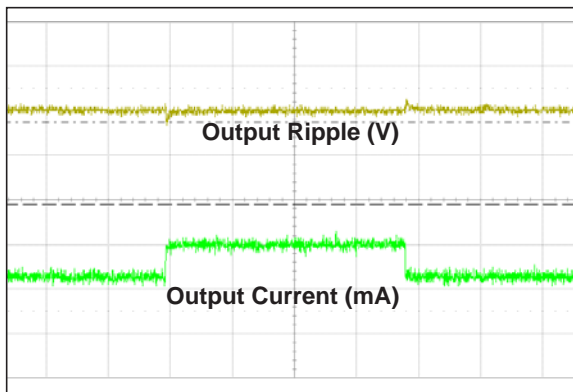
FIGURE 2-14: Load Transient Response ( I_{LOAD} = 50 mA/Div , Output: 100 mV/Div , Time: 100 \mu s/Div ).
