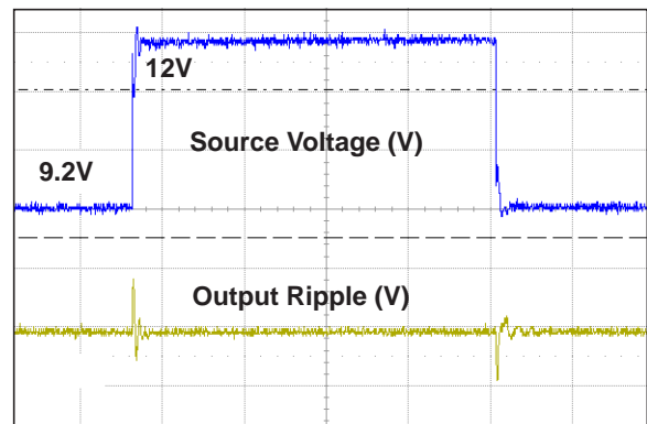
FIGURE 2-18: Line Transient Response ( I_{LOAD} = 100 mA , V_{IN} = 1V/Div , V_{OUT} = 100 mV/Div , Time: 100 \mu s/Div ).
