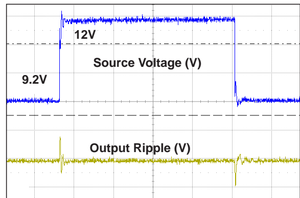
FIGURE 2-17: Line Transient Response ( I_{LOAD} = 10 mA , V_{IN} = 1V/Div , V_{OUT} = 100 mV/Div , Time: 100 \mu s/Div ).
