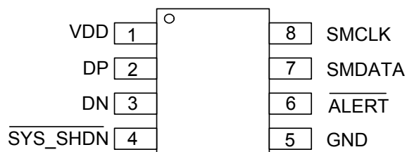
Figure 0.1 EMC1422 Pin Diagram
