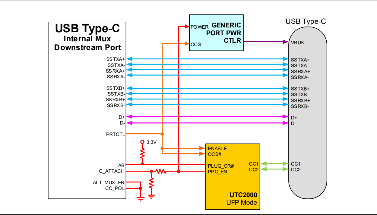
FIGURE 8-5: UFP TYPE-C PORT WITH GENERIC TYPE-C CONTROLLER & INTERNAL MUX (MODE 2)
