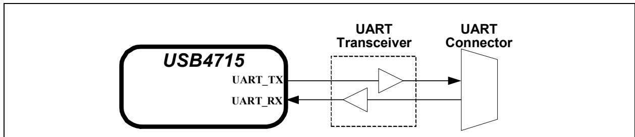
FIGURE 4-5: UART CONNECTIONS
