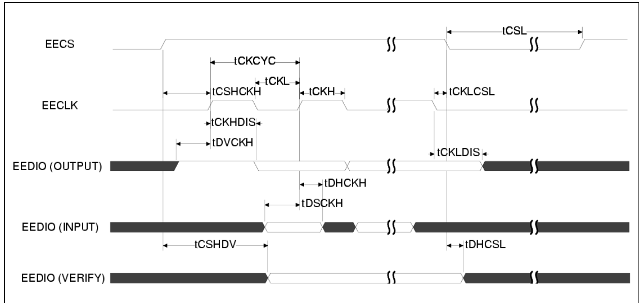
FIGURE 6-8: EEPROM TIMING
