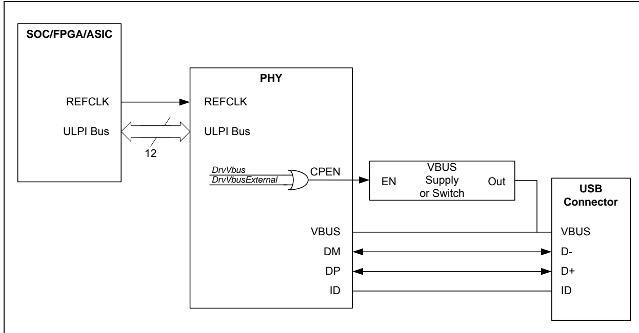
FIGURE 5-9: USB3318 DRIVES EXTERNAL VBUS SUPPLY OR SWITCH
