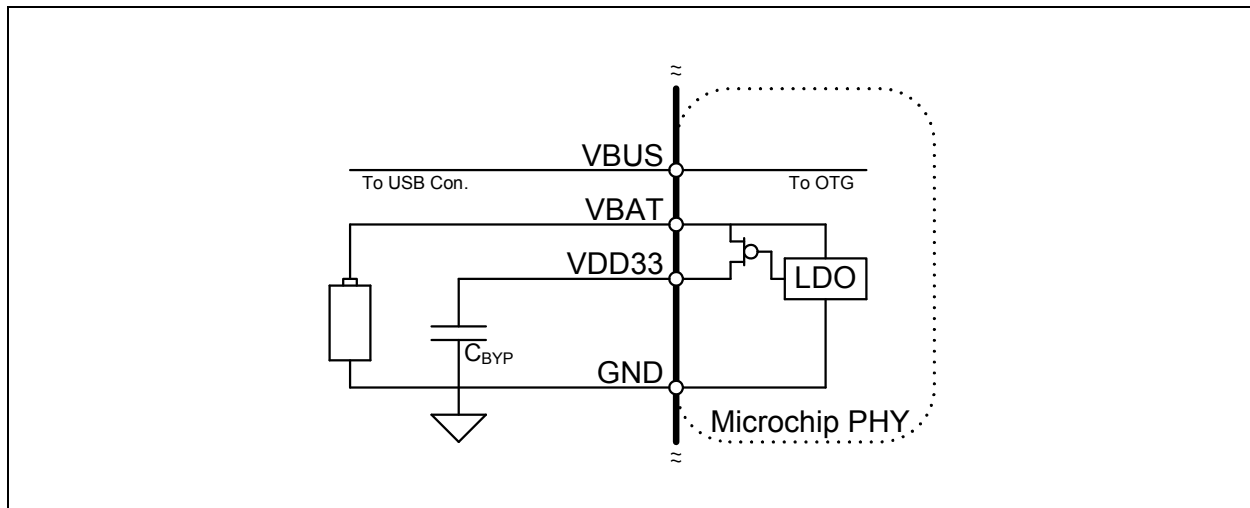
FIGURE 5-3: POWERING THE USB3318 FROM A BATTERY
