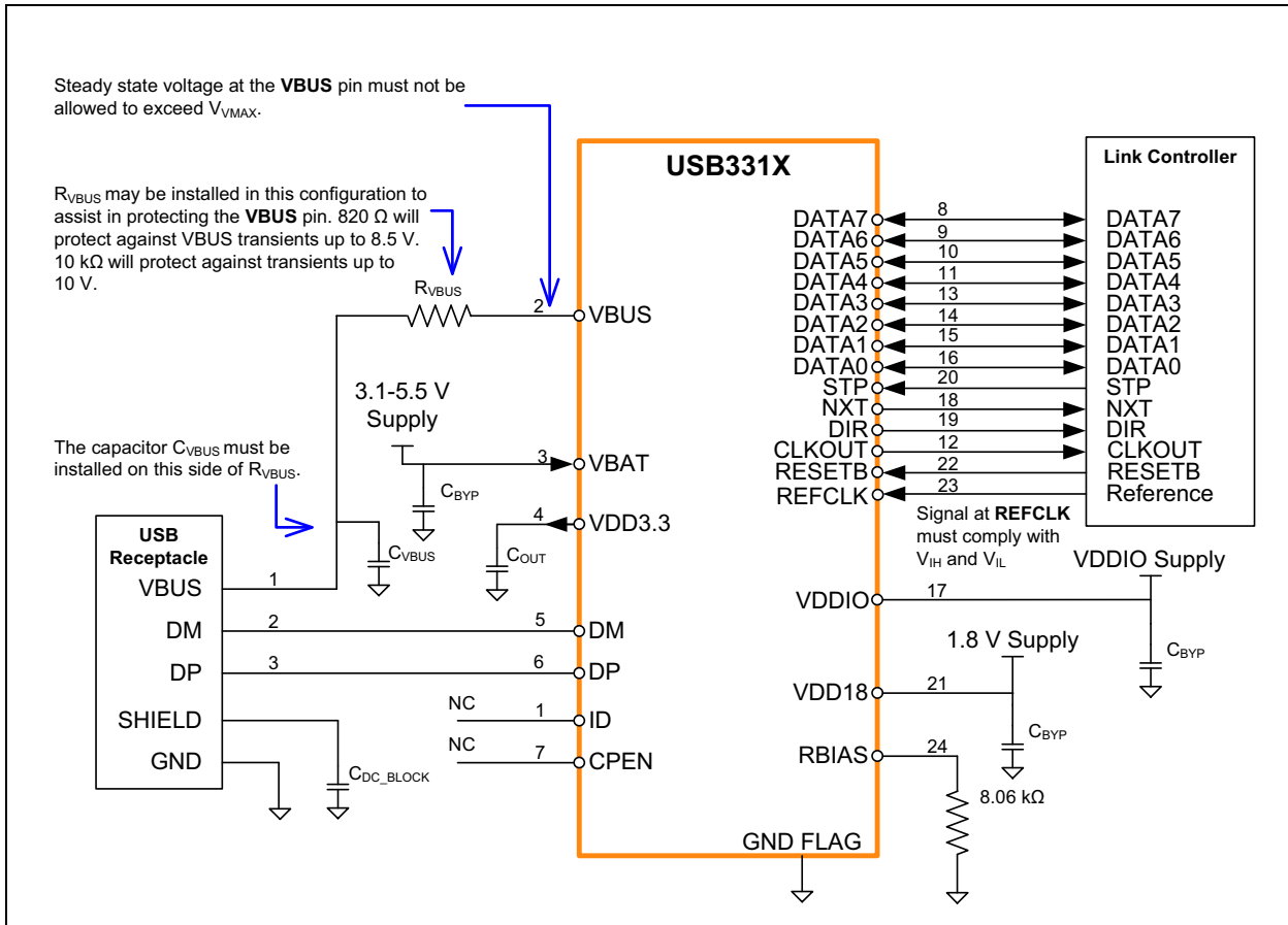
FIGURE 8-1: USB3318 QFN APPLICATION DIAGRAM (DEVICE)
