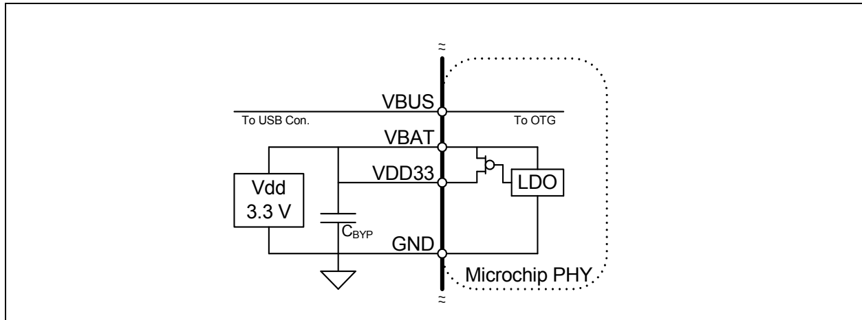
FIGURE 5-4: POWERING THE USB3318 FROM A 3.3 V SUPPLY
