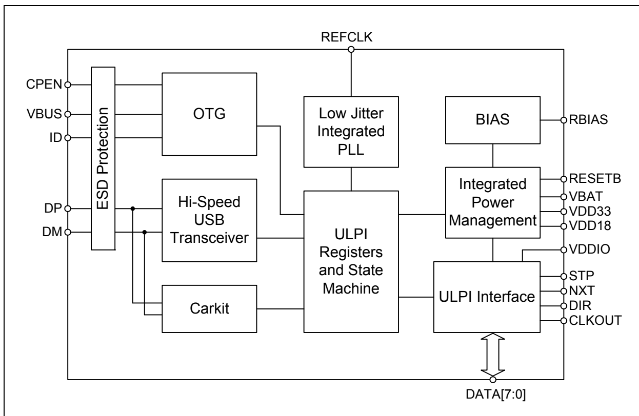
FIGURE 1-1: USB3318 BLOCK DIAGRAM
