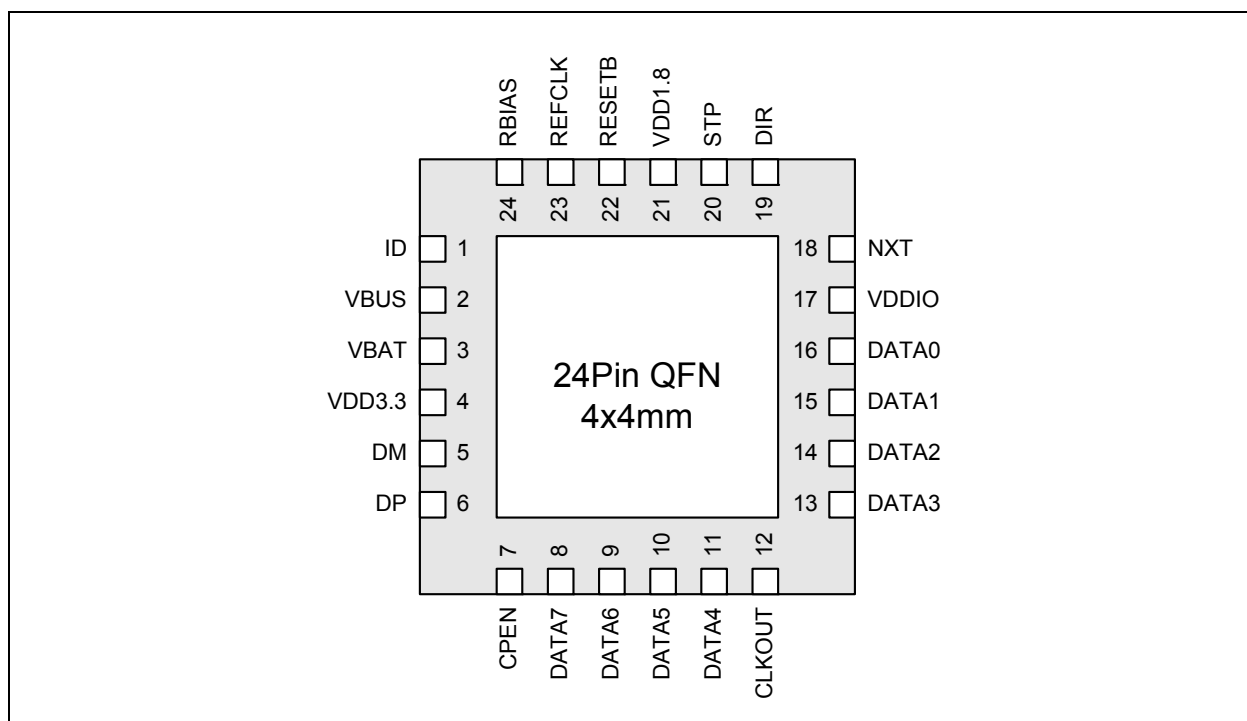
FIGURE 2-1: USB3318 QFN PINOUT - TOP VIEW
