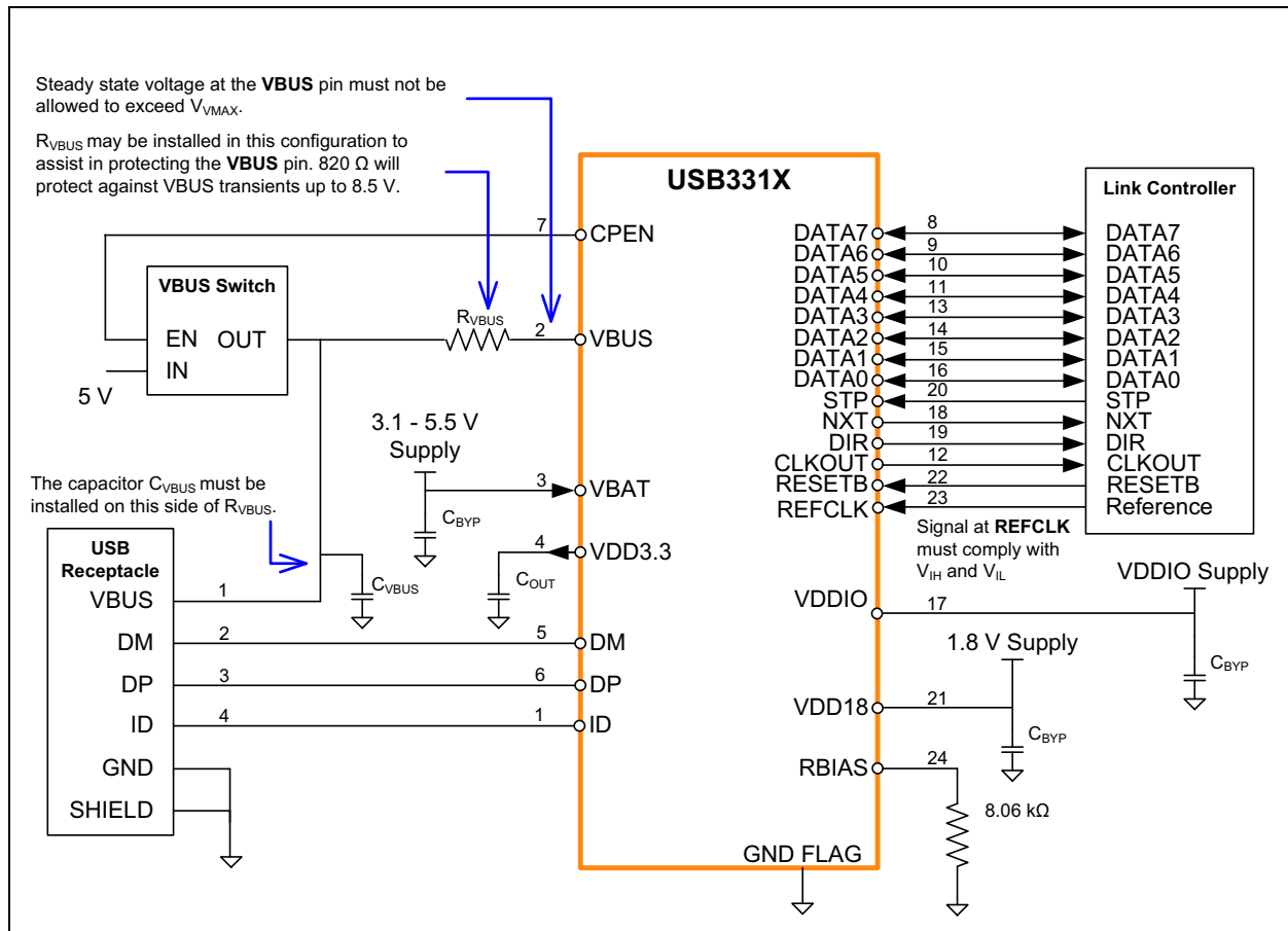
FIGURE 8-2: USB3318 QFN APPLICATION DIAGRAM (HOST OR OTG)
