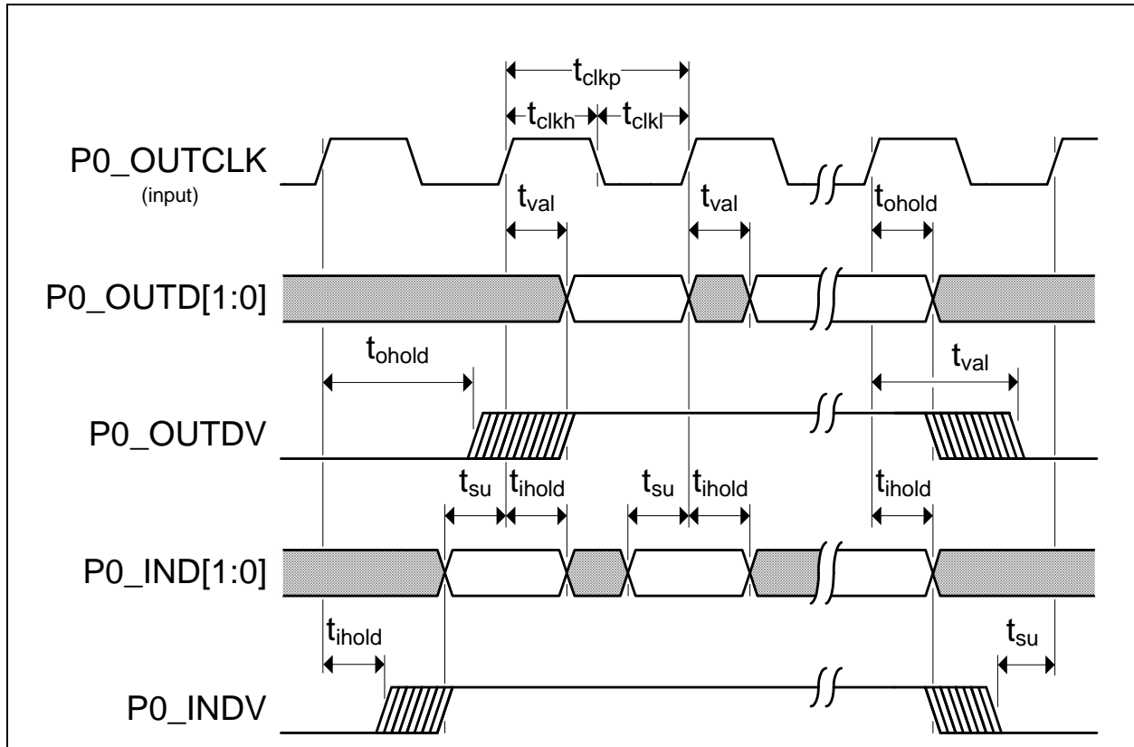
FIGURE 14-14: RMII P0_OUTCLK INPUT MODE TIMING
