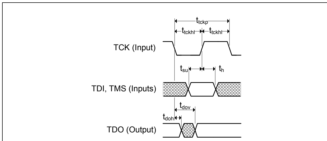
FIGURE 4-3: JTAG TIMING
