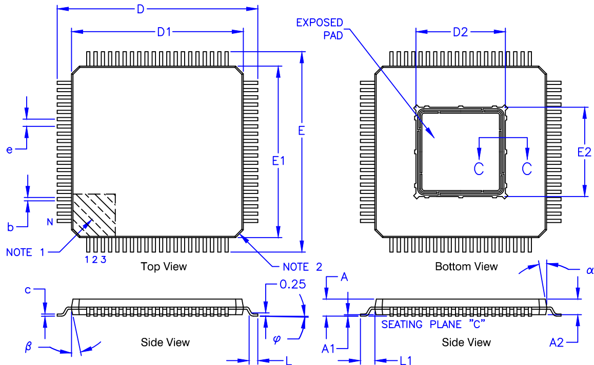
FIGURE 21-3: 80-TQFP-EP PACKAGE
