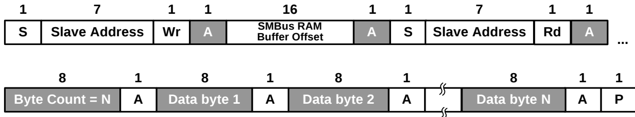
FIGURE 5-5: BLOCK READ
