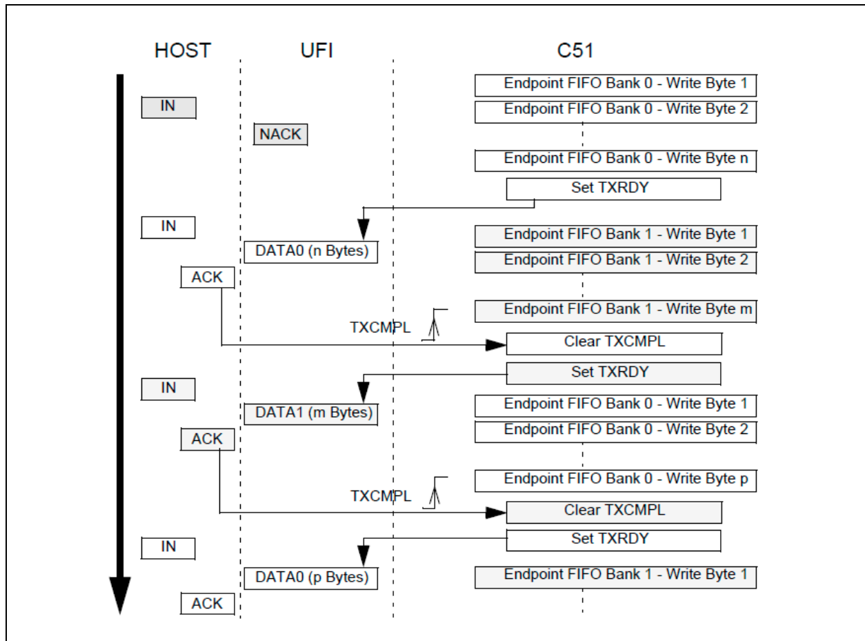
FIGURE 11-6: BULK/INTERRUPT IN TRANSACTIONS IN PING-PONG MODE
