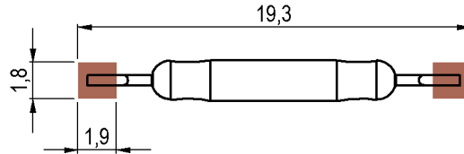
Recommended Pad Layout (mm) Unspecified Tolerances +/- 0,25mm
