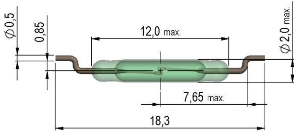
Dimensions (mm) Unspecified Tolerances +/- 0,25mm
