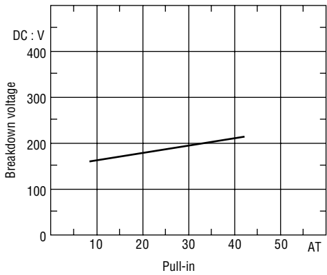
(3) Breakdown voltage
