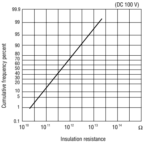
(4) Insulation resistance
