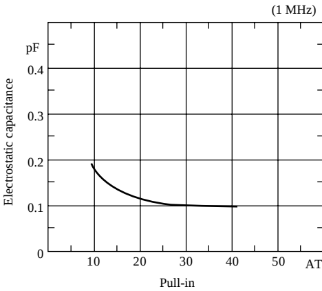
(5) Electrostatic capacitance
