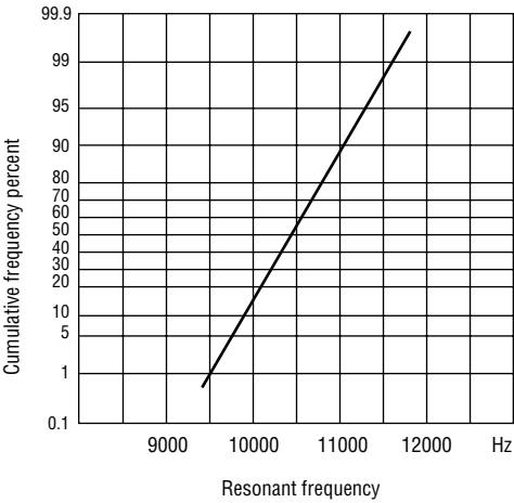
(4) Resonant frequency
