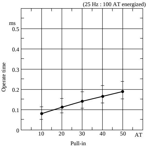
(1) Operate time
