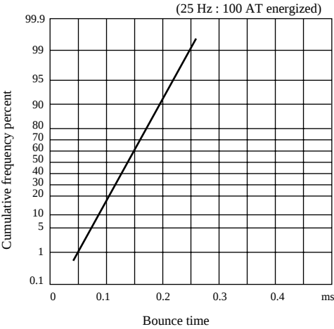
(2) Bounce time
