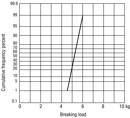
(2) Lead tensile strength
