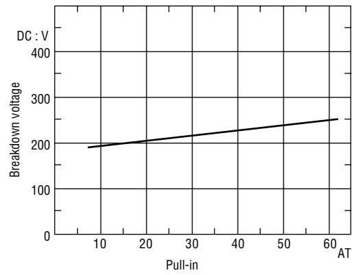
(3) Breakdown voltage
