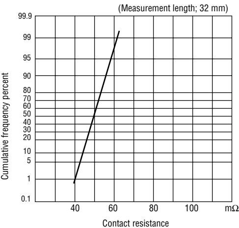
(2) Contact resistance
