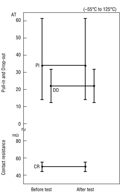
(2) Temperature cycle
