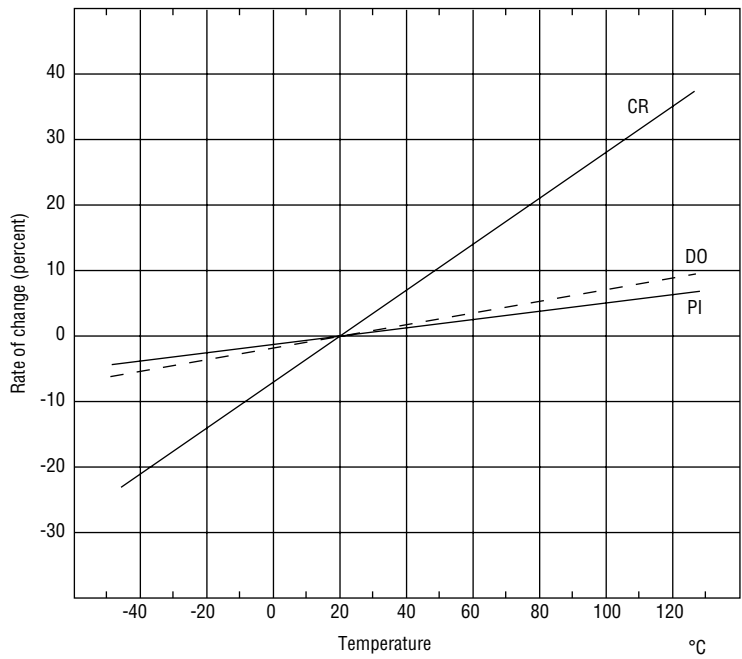
(1) Temperature characteristics
