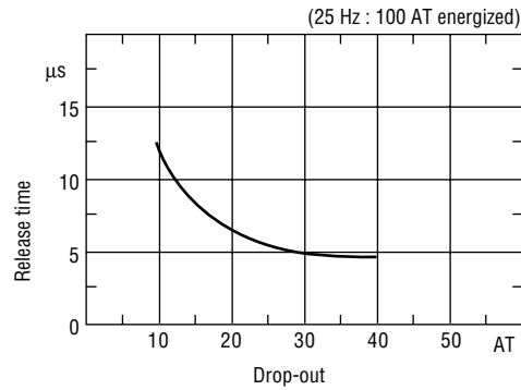
(3) Release time
