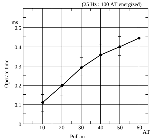
(1) Operate time
