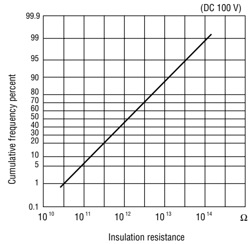
(4) Insulation resistance
