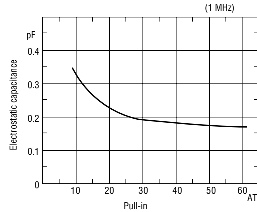
(5) Electrostatic capacitance
