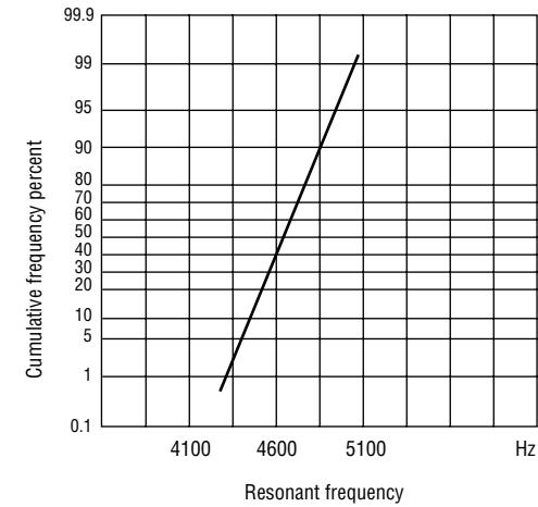
(4) Resonant frequency
