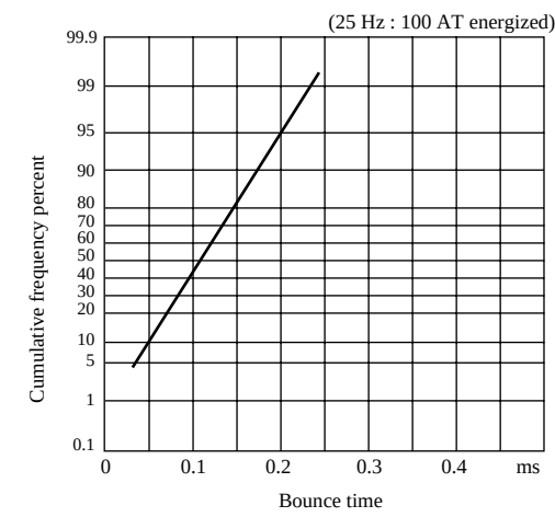
(2) Bounce time
