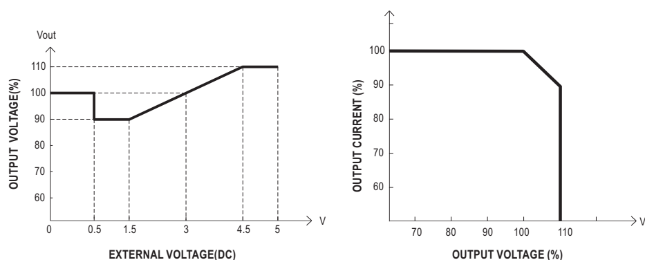
Fig. 2.2 Output voltage trimming
