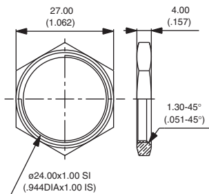
HEX NUT FOR MODELS Ø 24 (.944)
