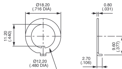
LOCKING RING
