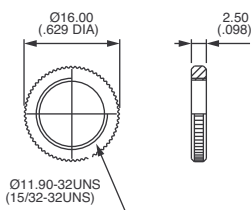
KNURLED NUT
