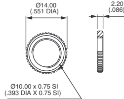
KNURLED NUT (std for 10400)
